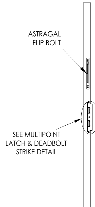
ASRAGAL STRIKE Multipoint Lock
