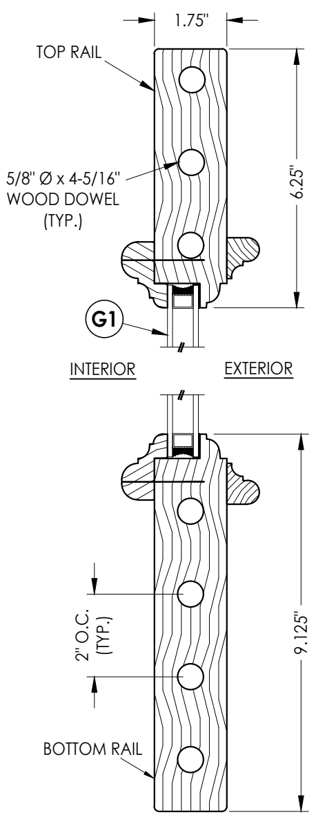
4 2 VERTICAL CROSS SECTION
