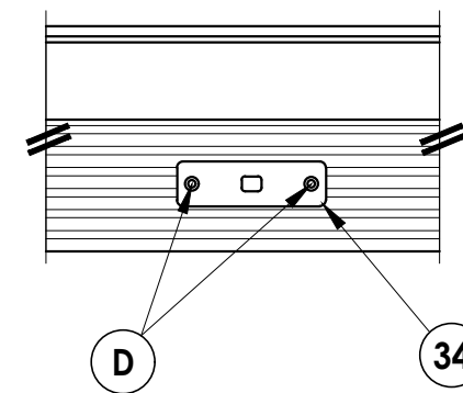
DETAIL 2 Astragal Shootbolt Strike Plate @ Sill (Outswing)
