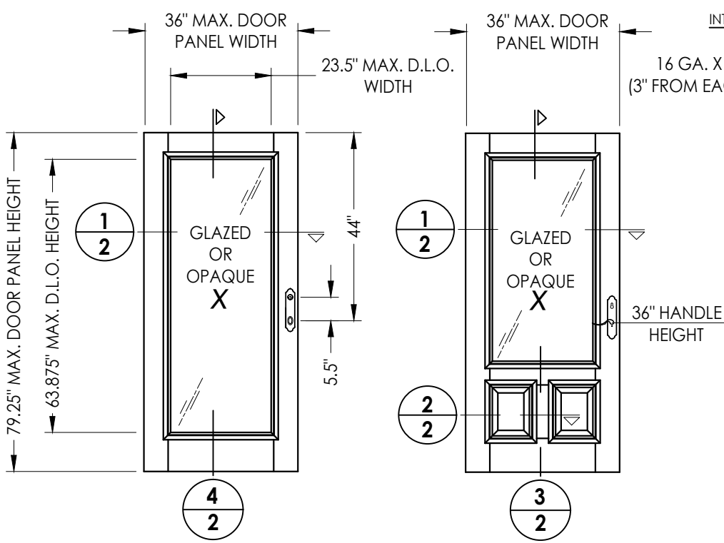
40 WOOD DOOR PANELS Glazed or Opaque
