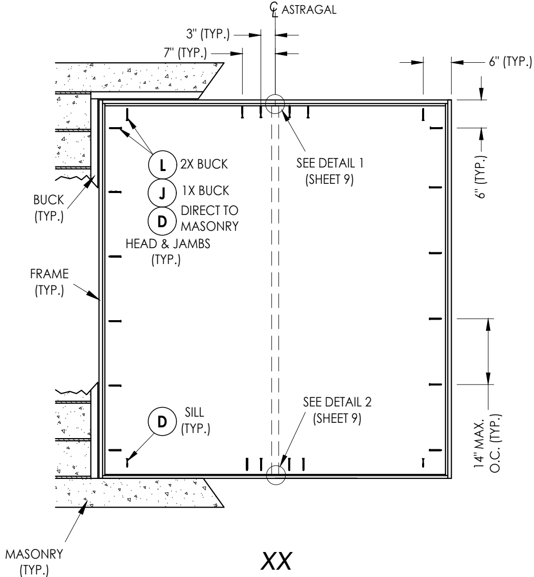
FRAME ANCHORING
